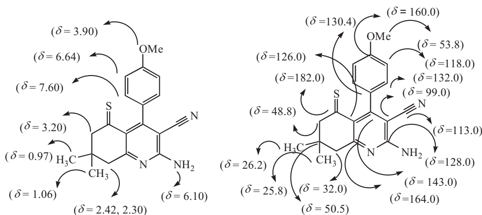
Fig. 1 Distinctive \delta 's values of compound 2a .
