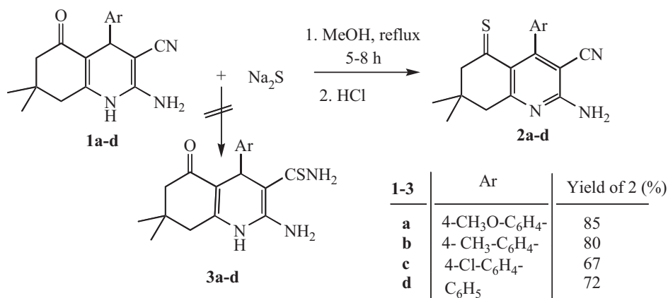
Scheme 1 Synthesis of tetrahydroquinoline-5-thiones 2a–d .
